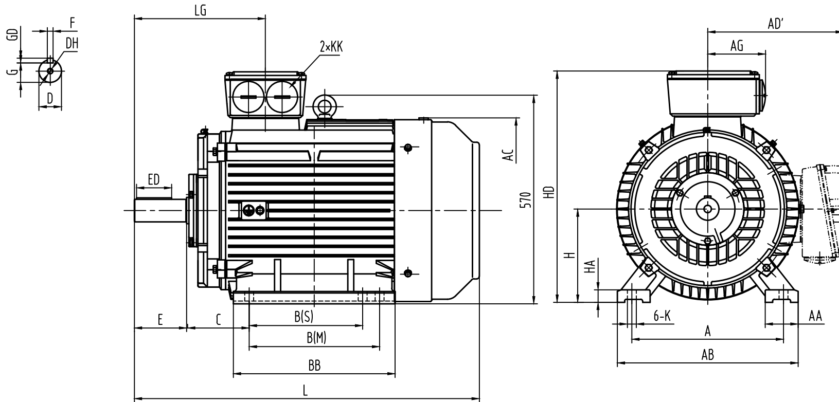
OUTLINE DIMENSIONS FOOT MOUNTED MOTORS
