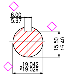
SECTION E-E
