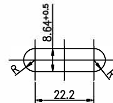
DETAIL AT 'A' SCALE 1:1
